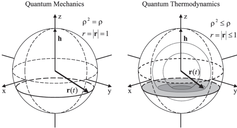
FIGURE 1. Pictorial representation for a two level system of the augmented state domain implied by the Hatsopoulos-Gyftopoulos kinematics with respect to the state domain of standard Quantum Mechanics. For a strictly isolated and uncorrelated two level system, quantum mechanical states are in one-to-one correspondence with the surface of the Bloch sphere, r = 1 ; quantum thermodynamical states are in one-to-one correspondence with the entire sphere, surface and interior, r \leq 1 .
